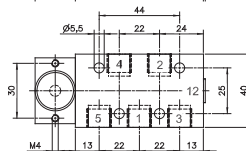
HV 53_701/HVR 53_701 HV 53_701 NPT/HVR 53_701 NPT
