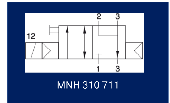
Alternative port-scheme "711"
