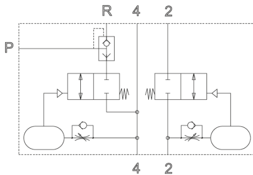
CBN 700 K Standard type
