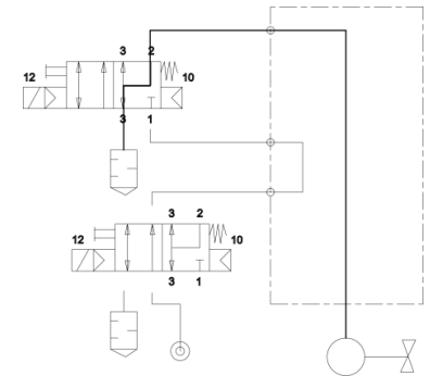
First valve not actuated, second valve actuated
