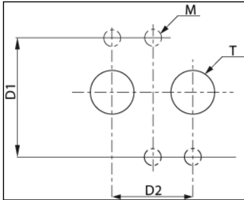
NAMUR-interface according to VDI/VDE 3845.
