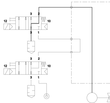
Both valves not actuated
