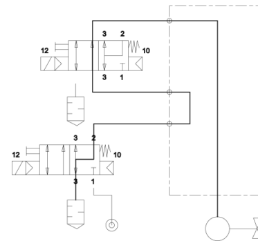
First valve actuated, second valve not actuated
