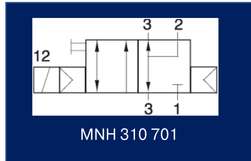
Standard port-scheme "701"
