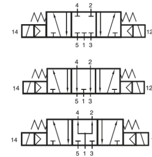
Centre closed
